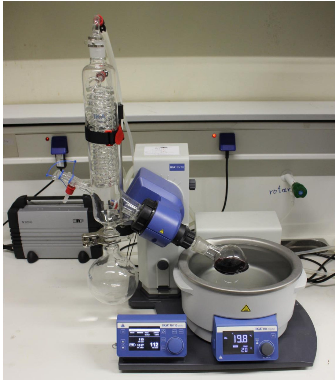
Rotary evaporator IKA RV10 with vacuum pump KNF N920G
