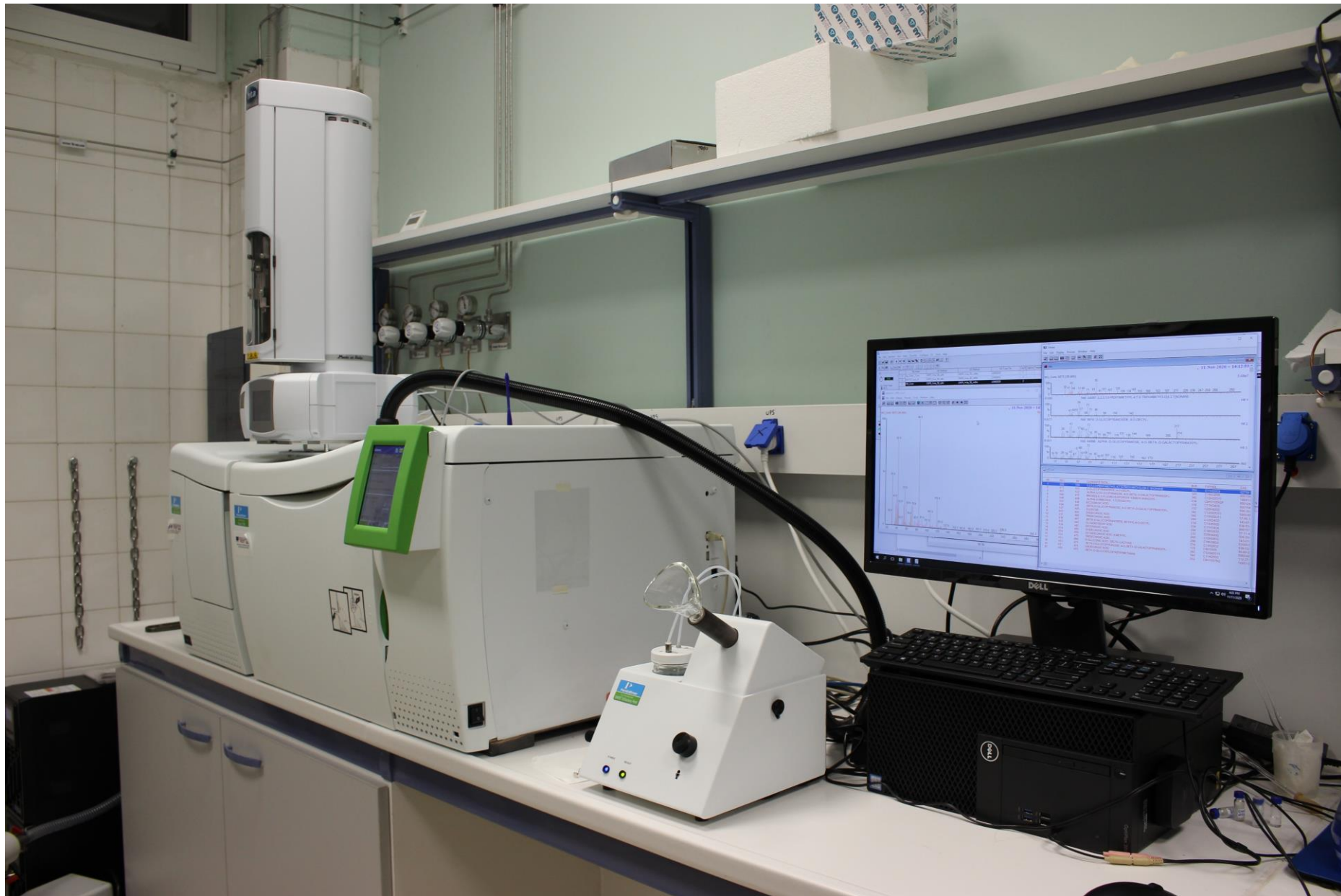
Gas Chromatography system Perkin Elmer Clarus 590 with MS detector Clarus SQ 8 S, SNFR Olfactory Port (GC-O) and autosampler HTA
