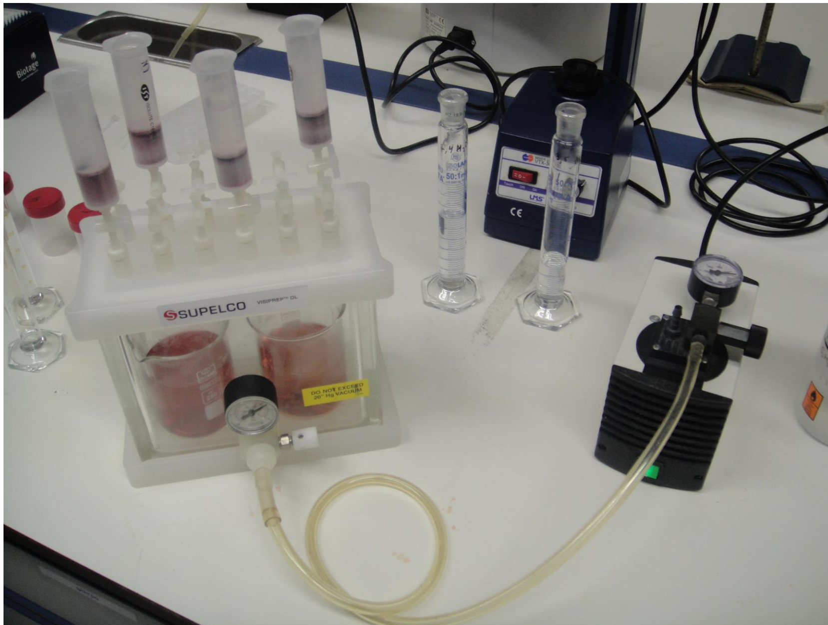
SPE extraction system (Visiprep™ SPE Vacuum Manifold, Supelco)
