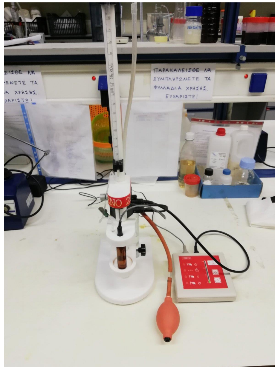
Titration ENO 20 PLUS (TDI) for the determination of Sulphur Dioxide
