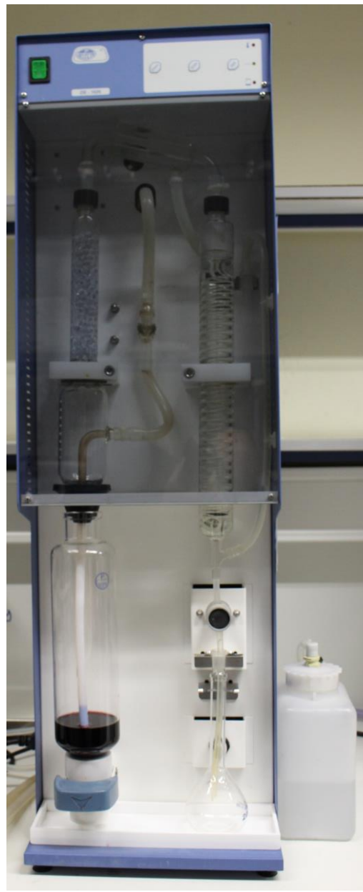
Oenological distillation unit Selecta DE-1626 for the determination of Alcohol Proof and the Volatile Acidity
